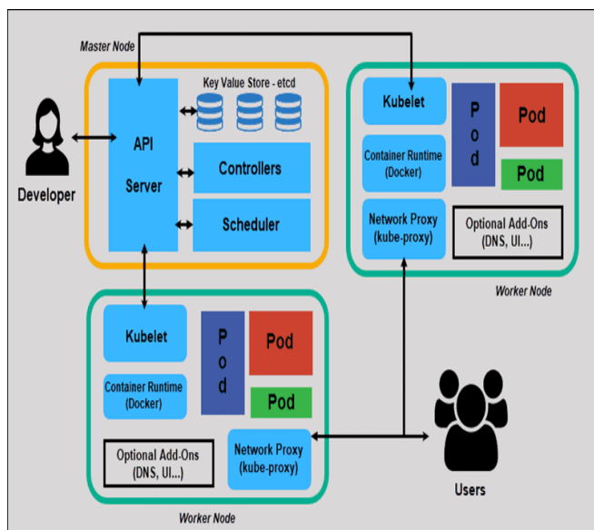
Fig.2 Kubernetes, Source:2
